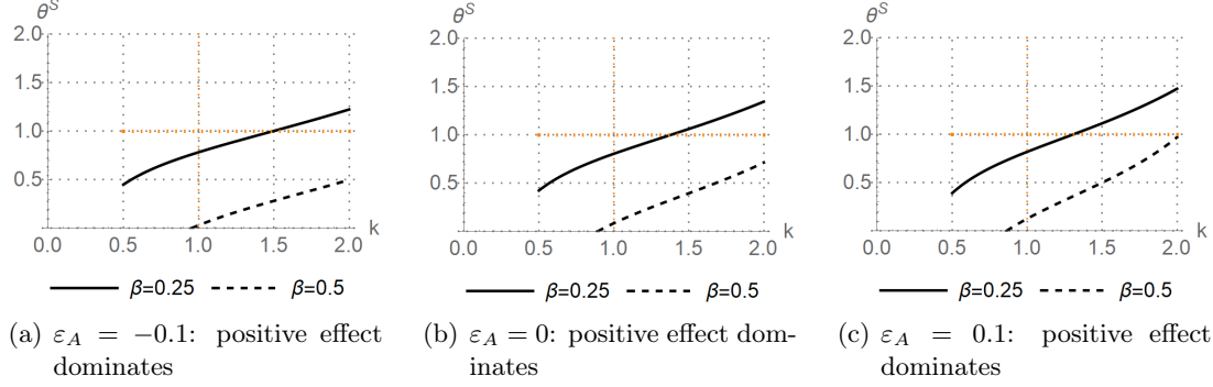
Figure 7: \theta^S(k, \dots, \epsilon_A, \beta, \dots) based on equation (24) for selected values of integration and scale; other parameters: l = 1 , n = l (which implies no impact of \epsilon_R ), \alpha = 0.5 . Notice that for n = l = k = 1 no symmetry results but \theta^S < k
